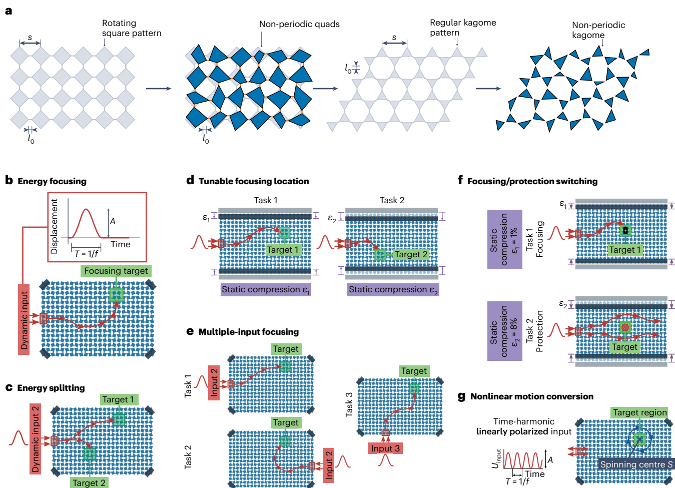
Fig. 1 | Inverse design of reprogrammable nonlinear dynamic metamaterials. a , Given a structure consisting of rigid units connected by flexible ligaments, such as a rotating-square pattern or a kagome pattern with spacing s and ligament length l_0 , the proposed framework optimizes the shapes of the rigid units to obtain a metamaterial design with the target nonlinear dynamic responses. b , The task of energy focusing, where the goal is to focus the energy provided by a dynamic excitation at a target region. A , amplitude; f , frequency; T , period. c , The task of energy splitting, where the goal is to split the energy provided by a dynamic excitation between two target regions. d , The task of tunable focusing location, where the goal is to reprogramme the energy-focusing
